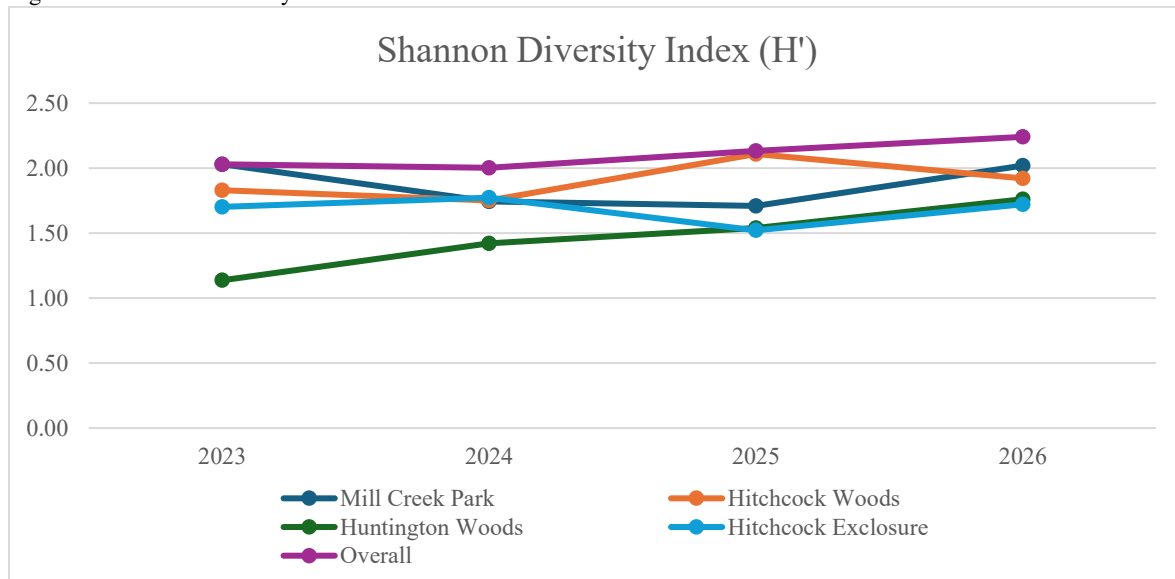
Figure 12. Shannon Diversity Index
