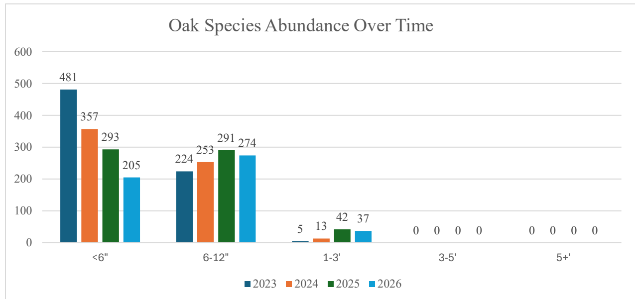
Figure 9. Oak Species Abundance Over Time
