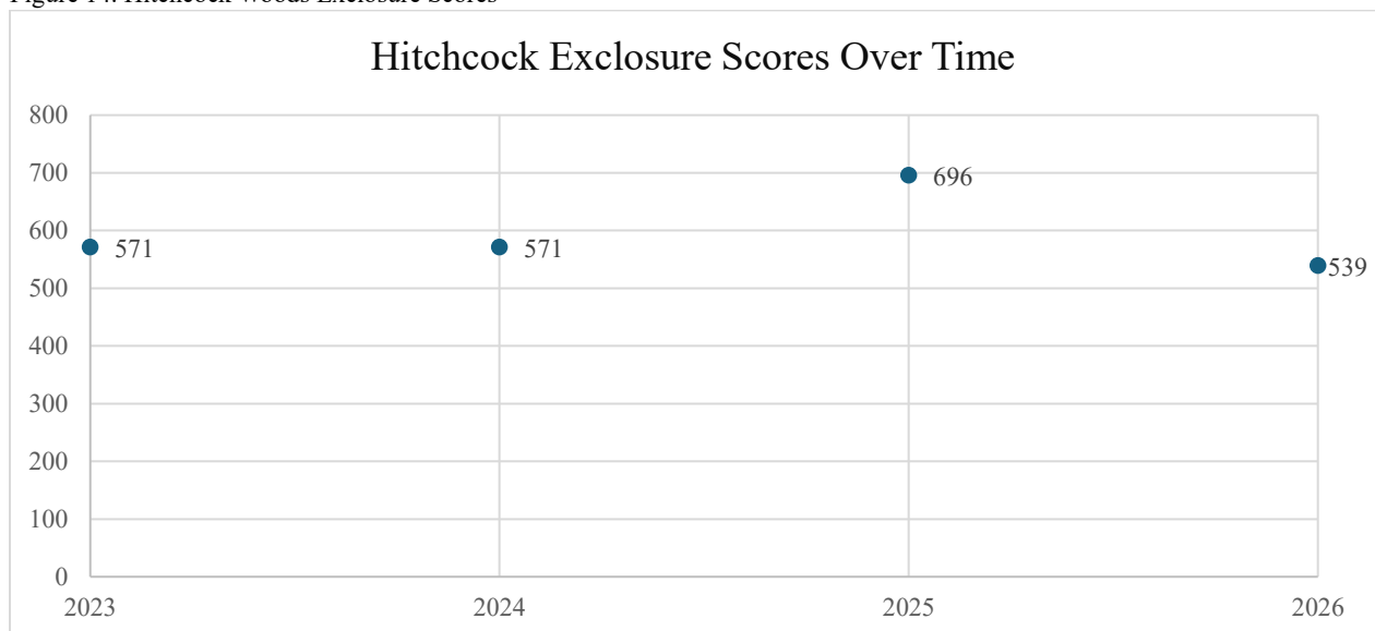
Figure 14. Hitchcock Woods Exclosure Scores
