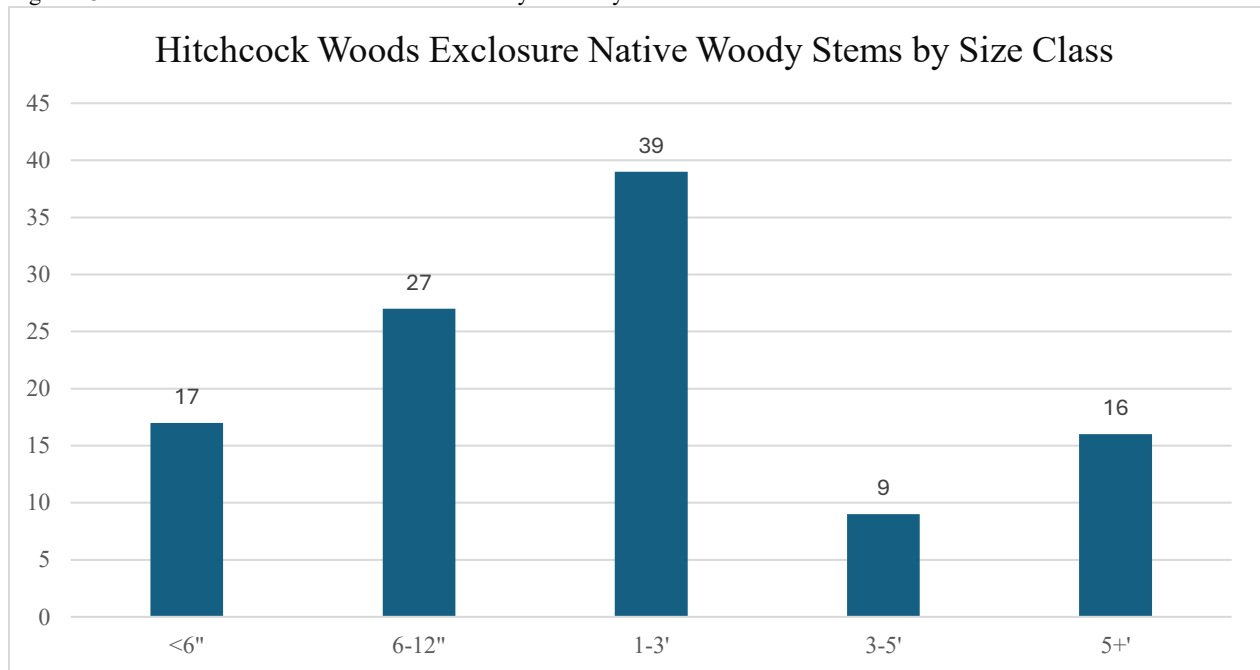
Figure 13. Hitchcock Woods Exclosure Native Woody Stems by size class
