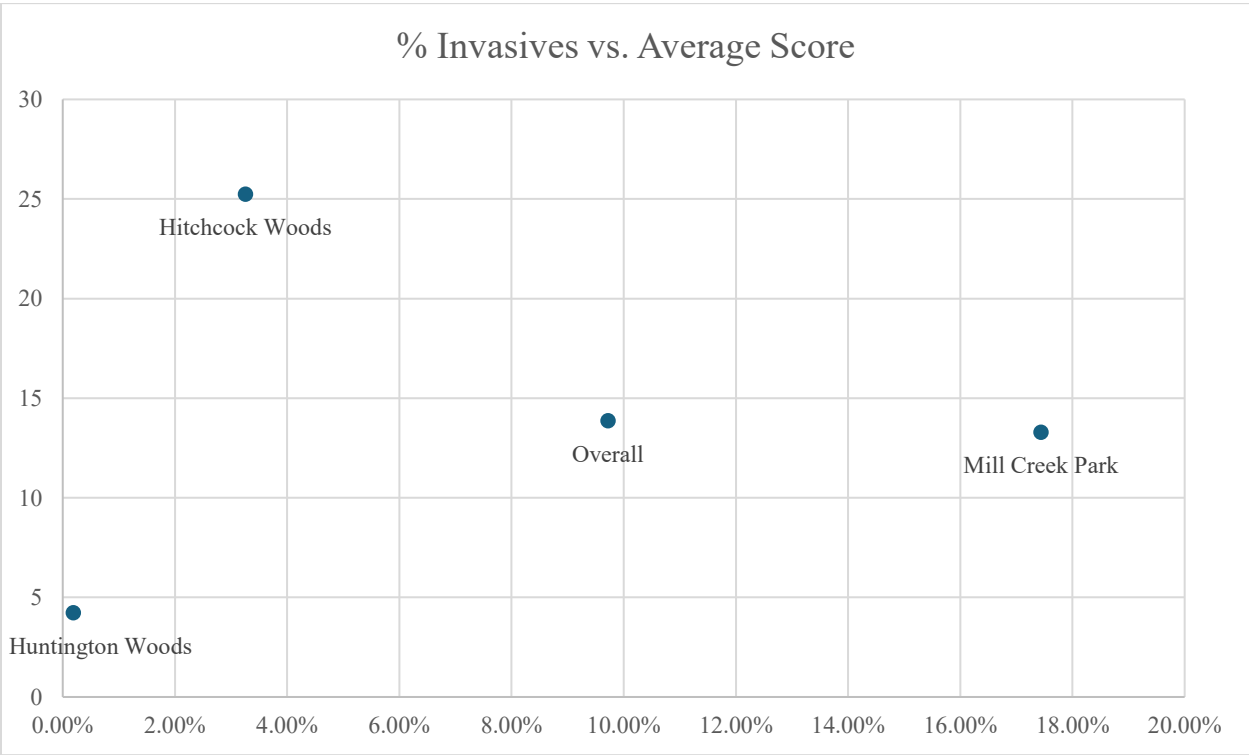
Figure 11. Percent of Invasives vs. Average Scores
