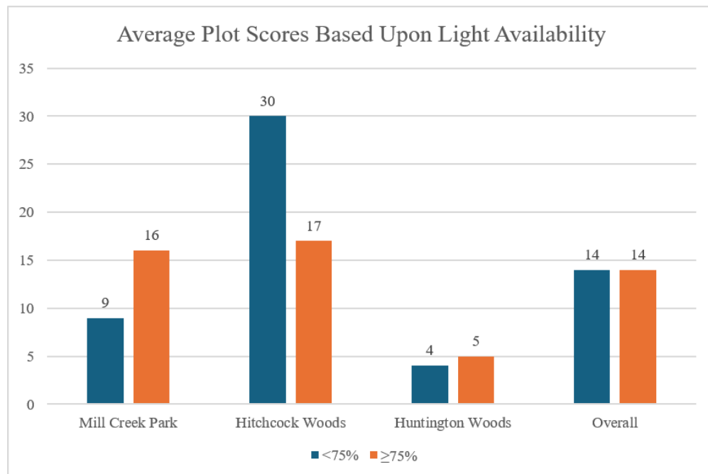
Figure 8. Average Plot Scores Based Upon Light Availability
