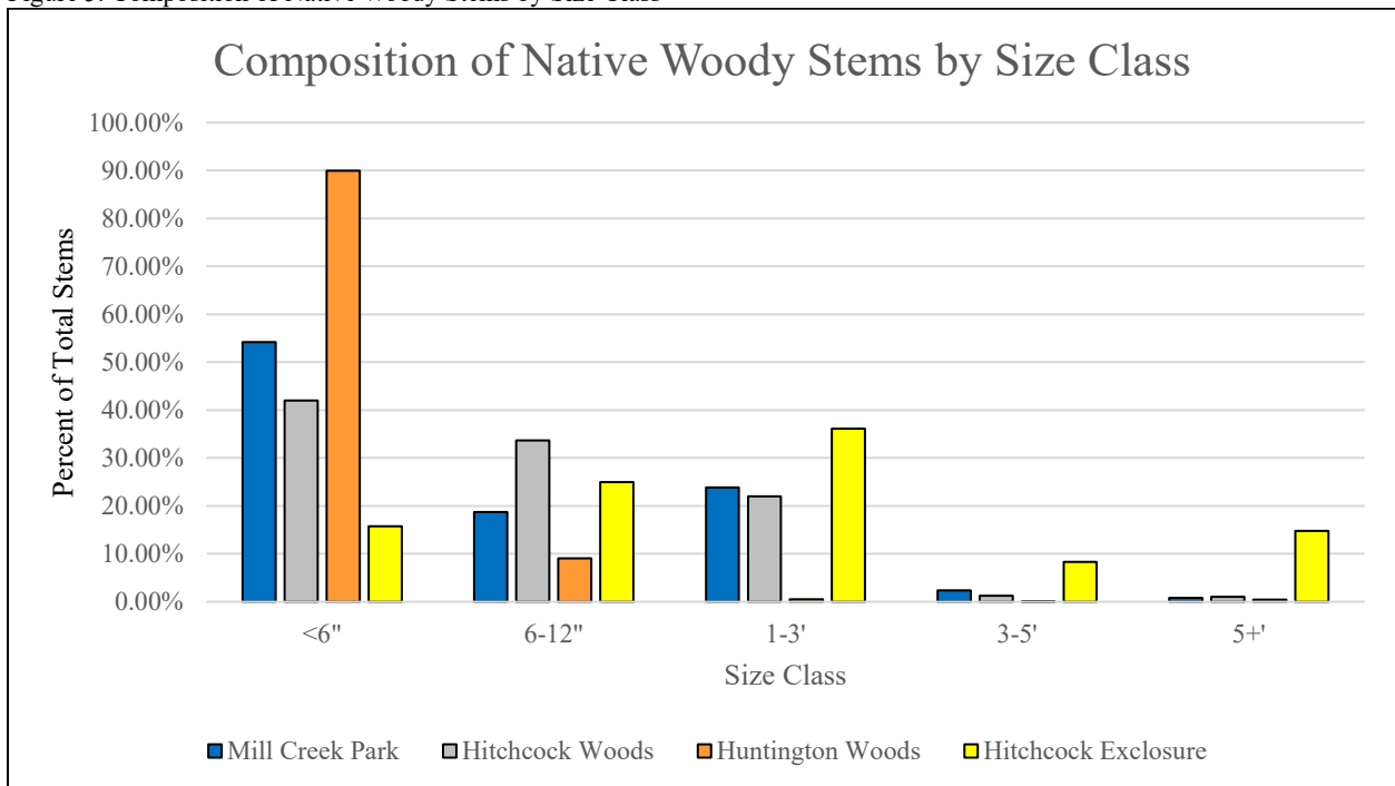
Figure 5. Composition of Native Woody Stems by Size Class
