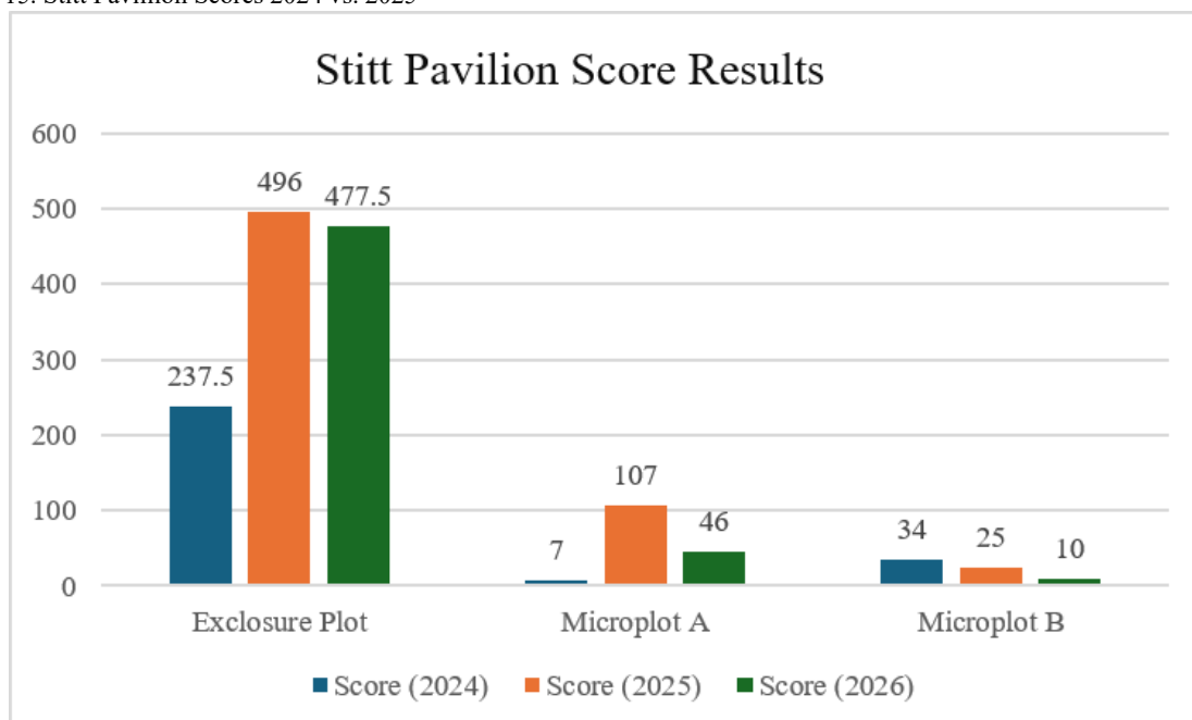
Figure 15. Stitt Pavillion Scores 2024 vs. 2025
