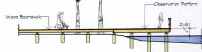
SECTION 'A' THROUGH NEW BOARDWALK TO LILY POND OBSERVATION PLATFORM
