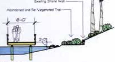
SECTION B THROUGH NEW BOARDWALK AT NE CORNER OF LILY POND
